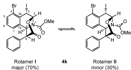
Scheme 1 Rotamers of compound 4k .
